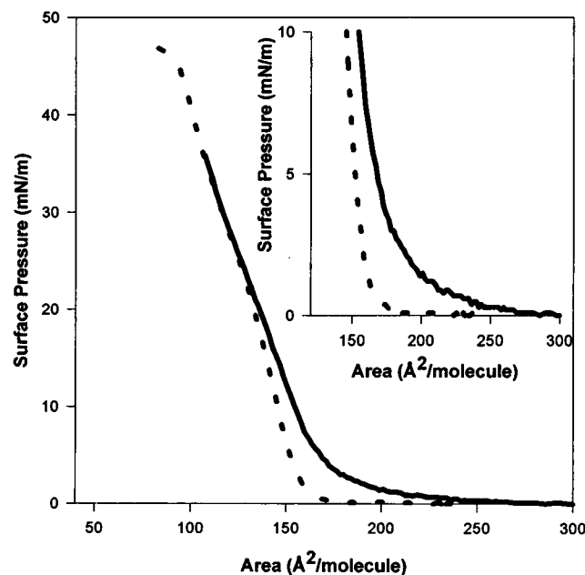
FIGURE 2 The \pi -A isotherm of a typical CF monolayer at 22°C, showing first compression (—) and recompression (---). The inset shows an expanded scale ( \pi \leq 10 mN/m) used for measuring A_{lo} .
